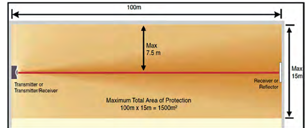
Maximum Area Coverage for Beam Detectors
